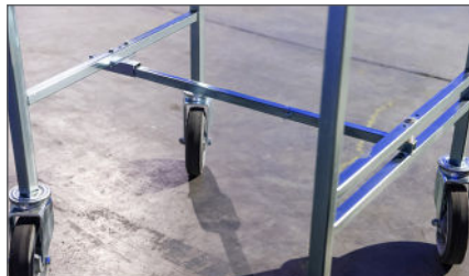
PERPENDICULAR LEG BRACE ON BOTH ENDS
